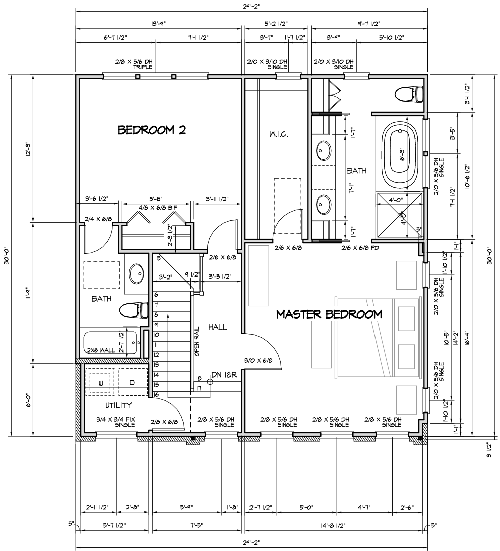
1 A-1 UPPER LEVEL 840 S.F. HEATED SCALE: 1/4"=1'-0"
